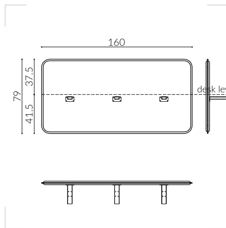
JAS.202.160x79.PG1.COLOR.MOTIVE
