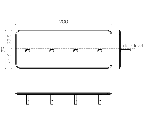
JAS.202.200x79.PG1.COLOR.MOTIVE
