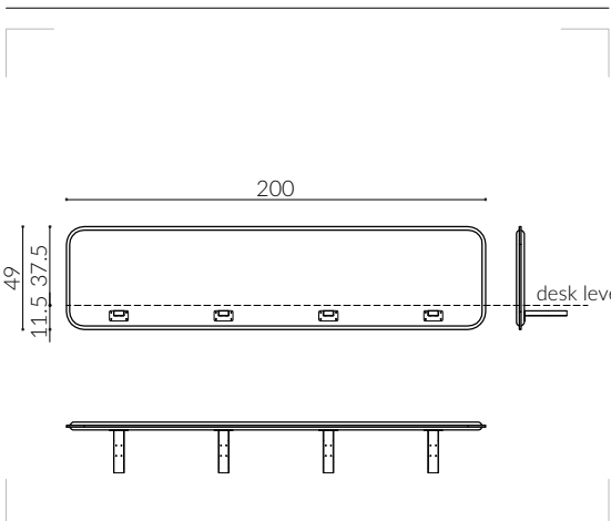
JAS.202.200x49.PG1.COLOR.MOTIVE
