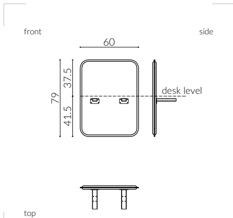
JAS.202.60x79.PG1.COLOR.MOTIVE
